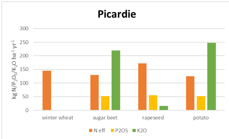
Figure 19: Fertiliser recommendation for Neff (efficient N), P 2 O 5 and K 2 O in Picardie on a silty soil. Displayed is the total demand which can be fulfilled partly with animal manure or other organic fertilisers.
