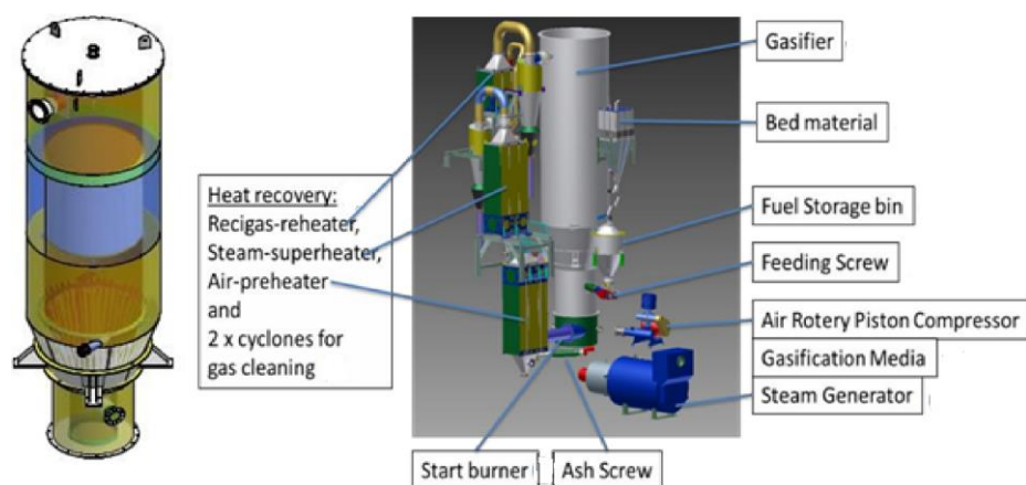
Figure 8. Overview of the gasification components at Soil Concept (Soil Concept, personal communication).
