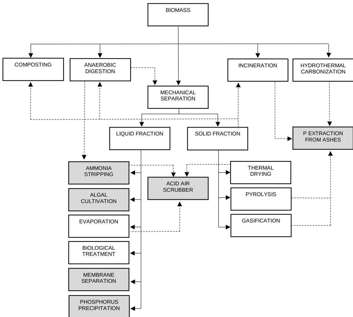
Figure 2. Overview of the biomass processing and nutrient recovery techniques (in grey)
