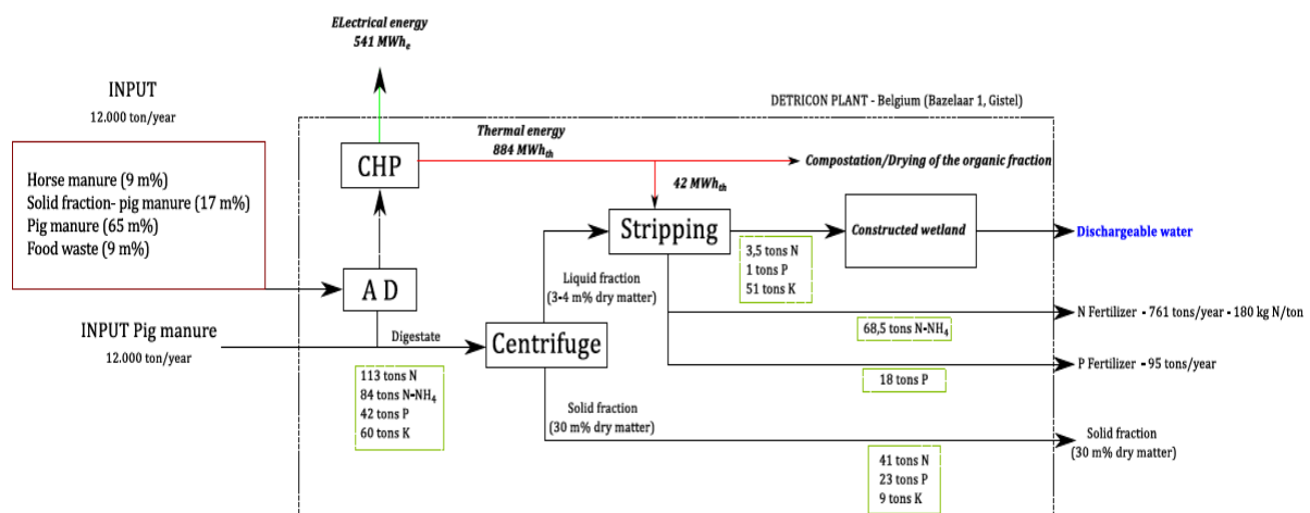
Figure 13. Schematic diagram of the nutrient recovery and reuse technology involving anaerobic digestion (AD) and \text{NH}_3 stripping/scrubbing by Detricon (Detricon, personal communication).
