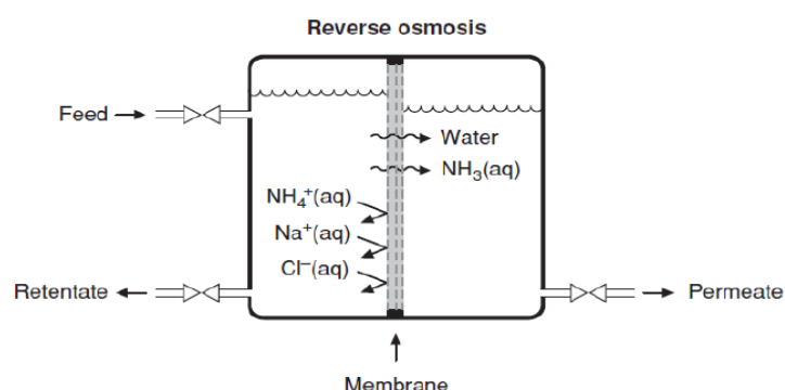
Figure 11. Reverse osmosis filtration for concentration of ions in liquid manure (Christensen et al., 2013).
