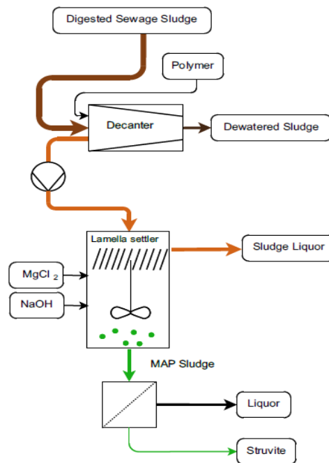
Figure 12. Process scheme of the STRUVIA™ struvite crystallization by Veolia Water (P-REX, 2015b).
