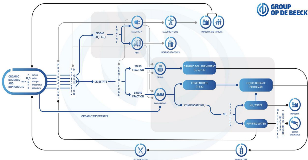
Figure 14. Schematic diagram of the nutrient recovery and reuse technology at Group op de Beeck (Group op de Beeck, 2019)
