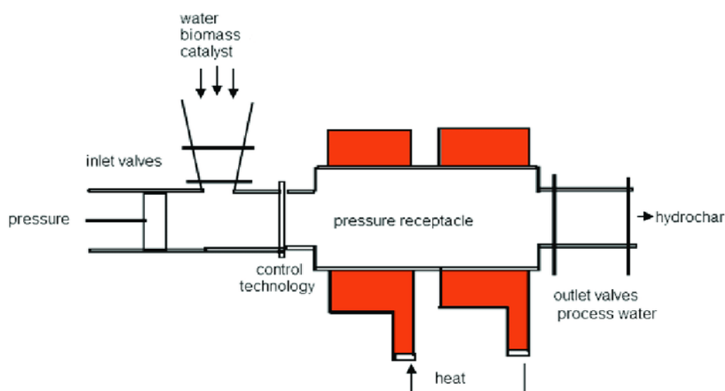
Figure 5. A diagrammatic representation of a HTC reactor (principal components of the Artec Hydrothermal Carbonization plant) (Glaser, 2015).
