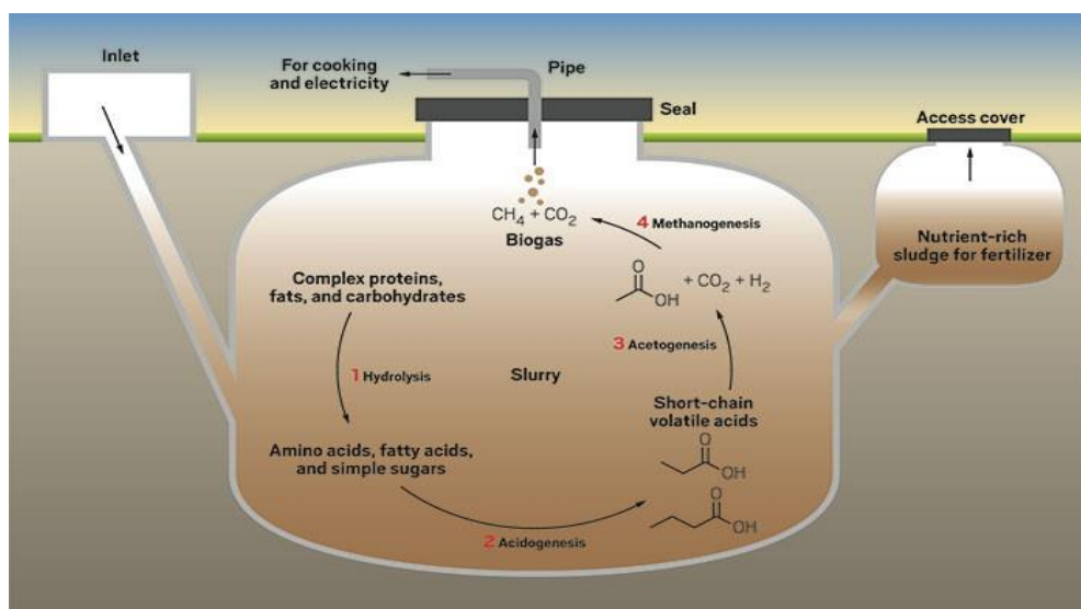
Figure 3. A diagrammatic representation of the processes in an anaerobic digestion (AD) unit (Lim, 2016).
