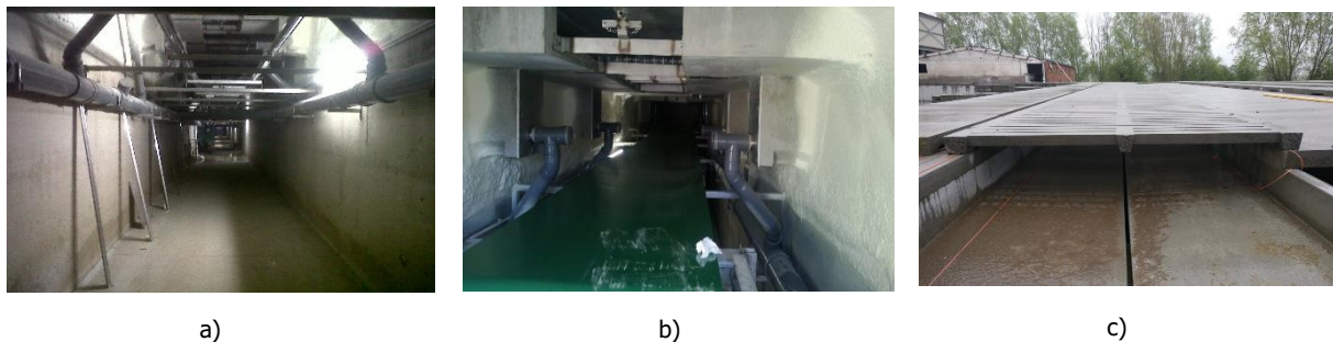
Figure 6. The VeDoWS system for manure separation: a) pipeline which collects urine from all the stable units; b) conveyor belt to transfer the SF from the slatted floor to the manure storage area; c) gutter for urine collection (Vermeulen Construct, n.d.).
