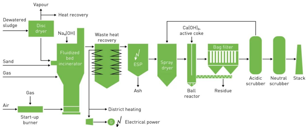
Figure 4. Diagrammatic representation of the Outotec sewage sludge incineration plant 100 (Outotec, n.d.)
